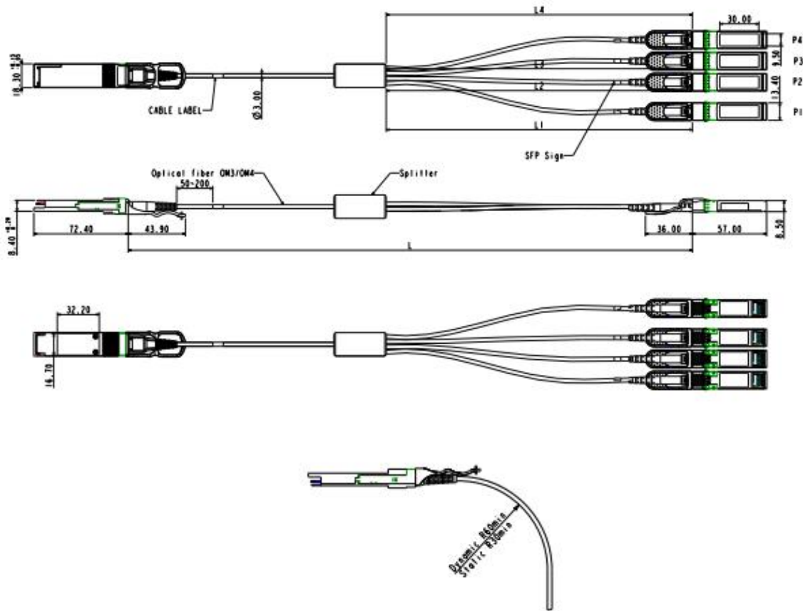
Figure1. Mechanical Specifications
